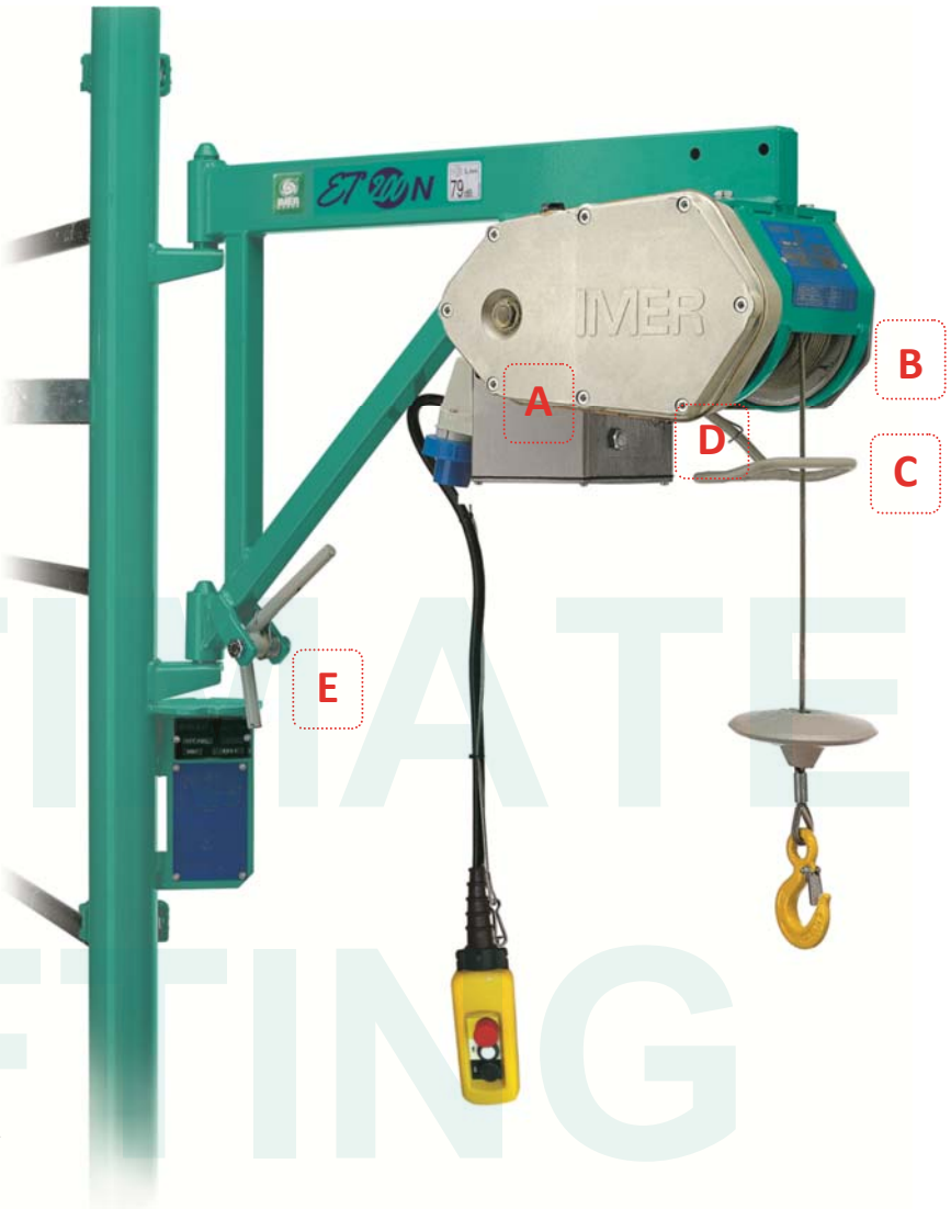
C UPPER LIMIT SAFETY DEVICE
